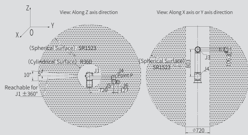
AUBO-i20 Moving Range of Point P
