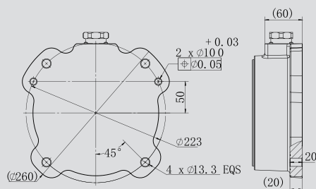
AUBO-i20 Top View of Base
