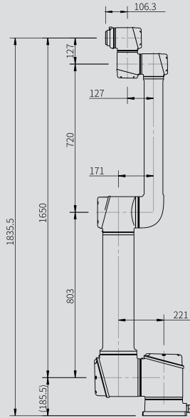
AUBO-i20 Dimensions
