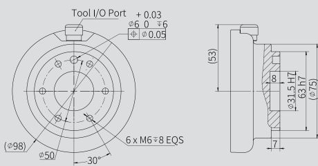
AUBO-i20 Tool End Flange
