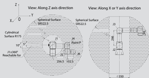
AUBO-i3 Moving Range of Point P
