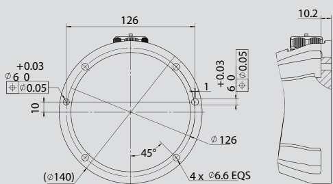
AUBO-i3 Top View of Base
